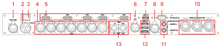
grandMA3 full-size CRV rear panel
